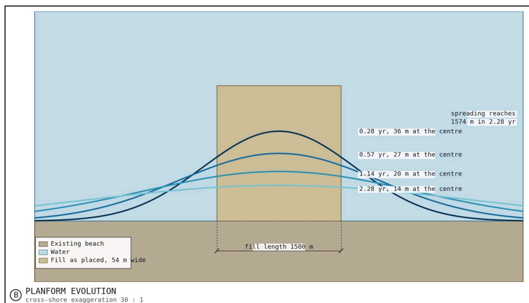
Figure 20.4: Nourishment module, planform view.
