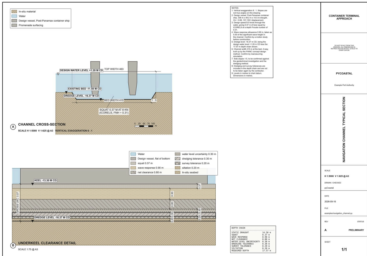
Figure 19.3: Navigation channel with true-scale keel detail (channel1_sheet).
