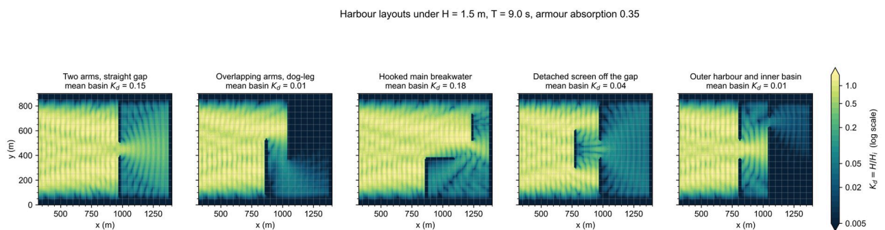
Figure 11.2: The five built-in layouts under the same design wave.
