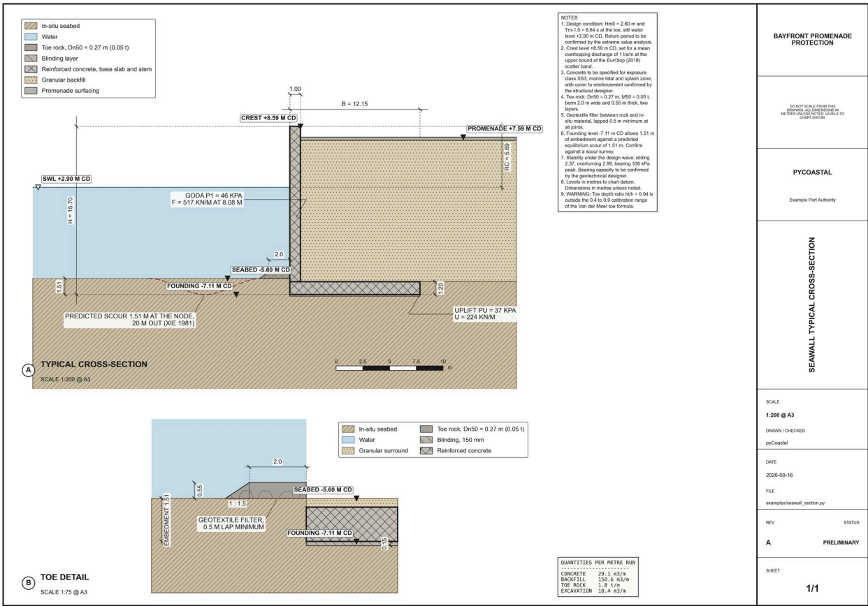
Figure 10.1: The seawall drawing sheet: typical section at a true stated scale, an enlarged toe detail, the design parameter block, and specification notes generated from the design.
