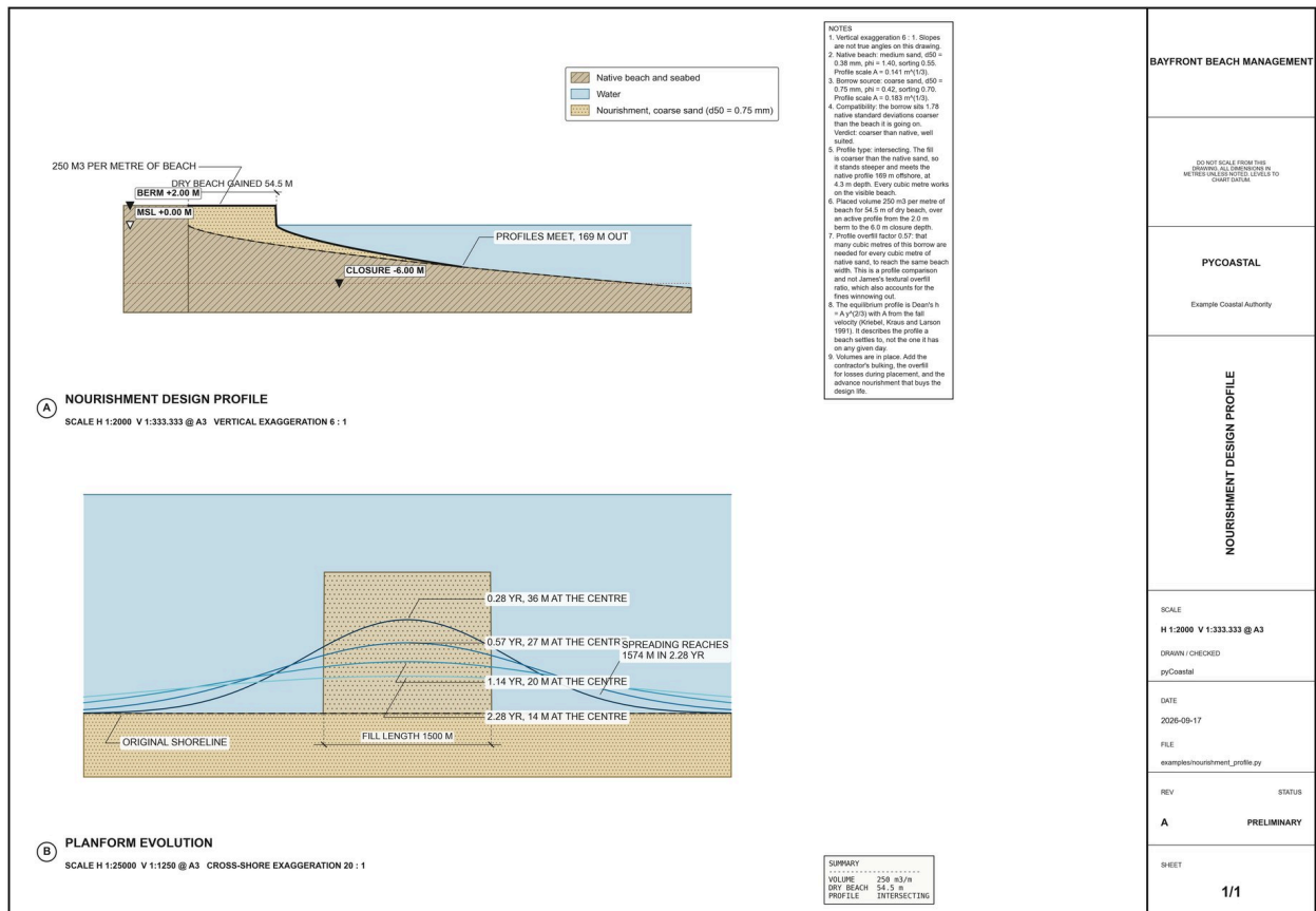
Figure 17.5: Nourishment drawing sheet with the design profile and the planform on one sheet, each at its own standard scale.
