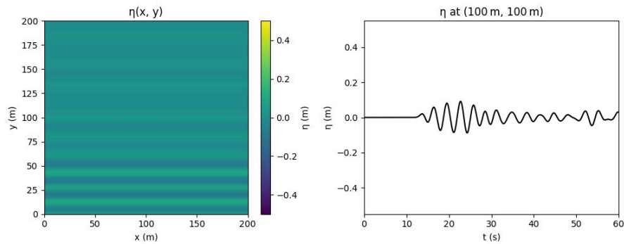
Figure 5.2: Irregular wave field at the end of the run (examples/wave2D_irregular.py).
