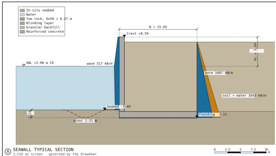
Figure 20.1: Seawall module sheet as rendered by draw.js.
