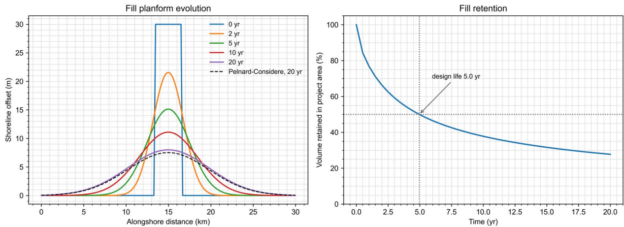
Figure 17.1: Nourishment design study: planform evolution against the Pelnard-Considere solution, retained volume, and the renourishment cycle.
