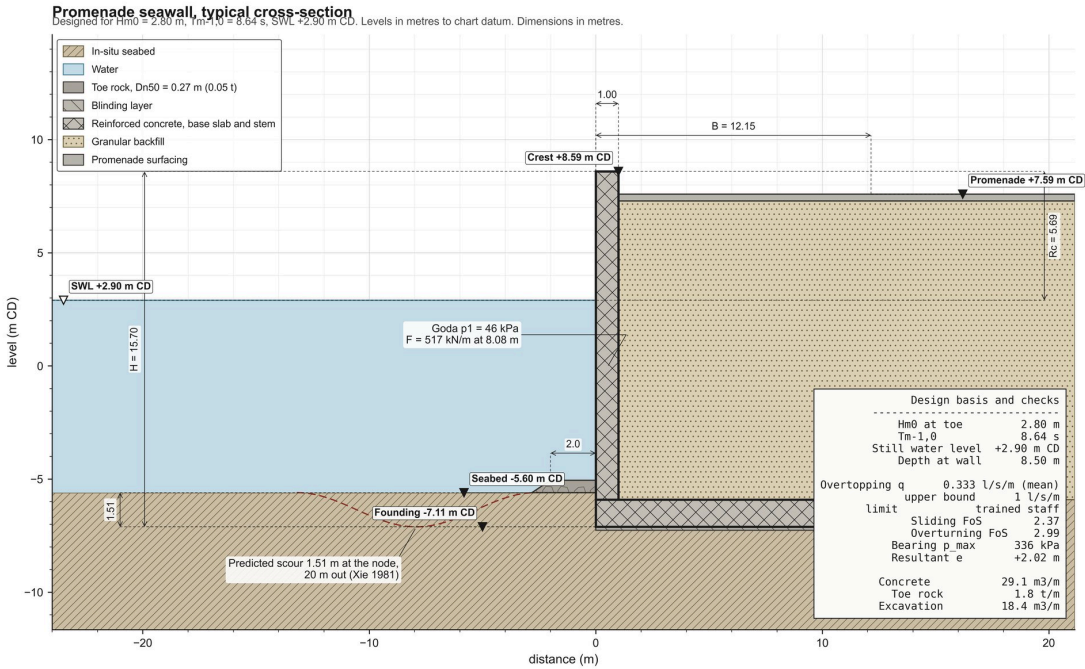
Figure 10.2: Standalone seawall section with plot axes, for a report.
