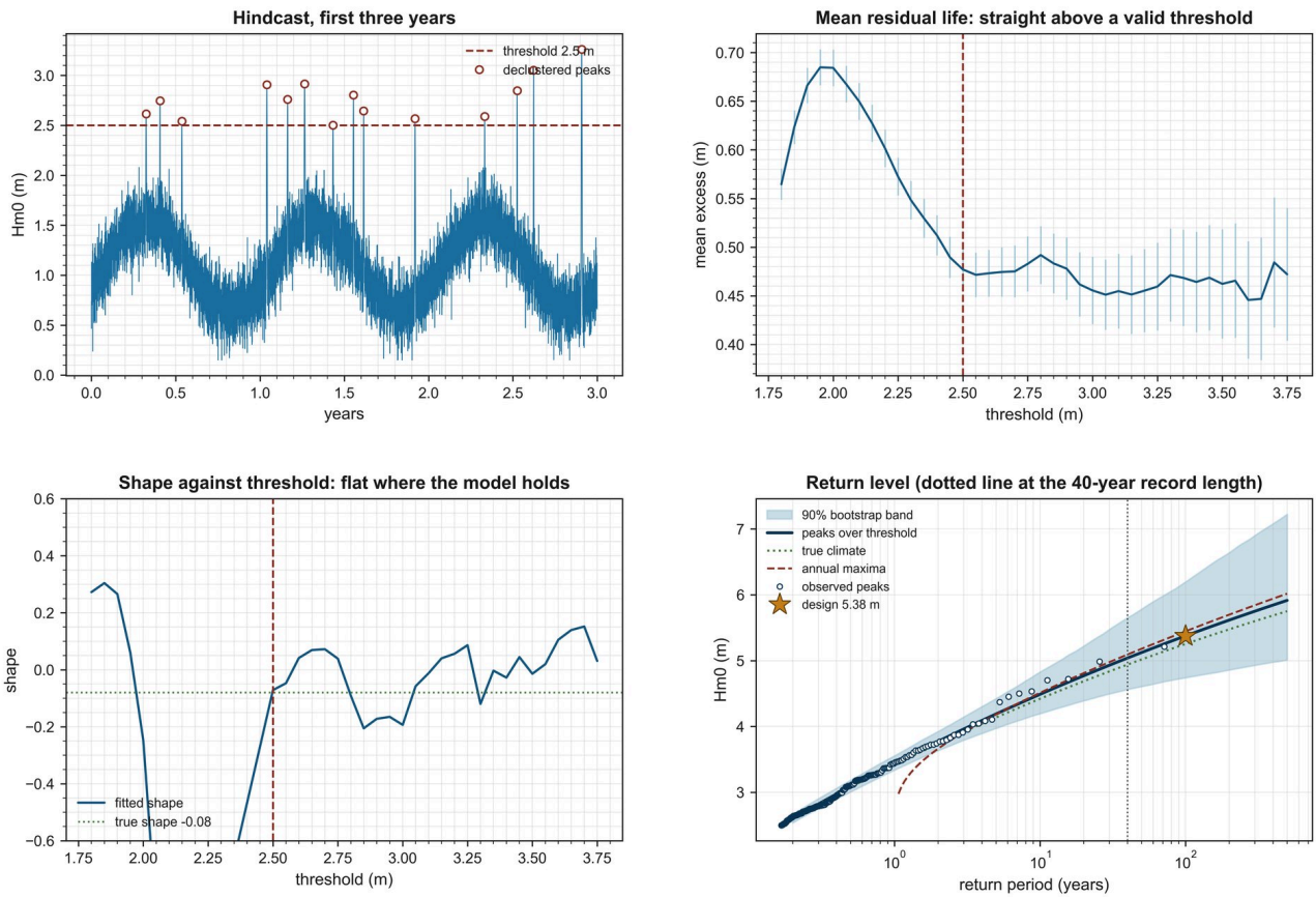
Figure 7.1: Extreme value analysis of a 40-year record: threshold diagnostics, return level plot with bootstrap band, and the sampling spread of the 100-year estimate.
