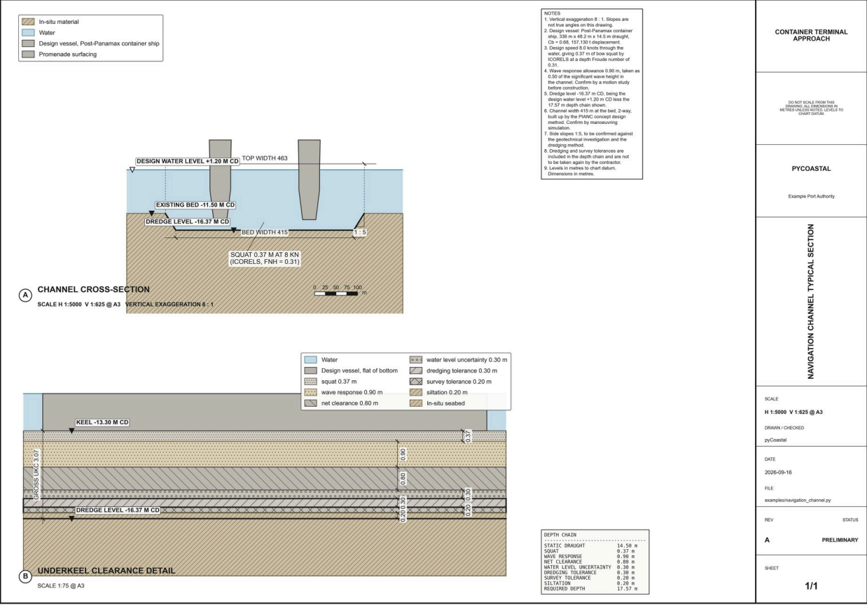
Figure 15.1: Navigation channel drawing sheet: the whole channel with a stated vertical exaggeration, and the underkeel clearance at a true scale where the allowances read as real thicknesses.
