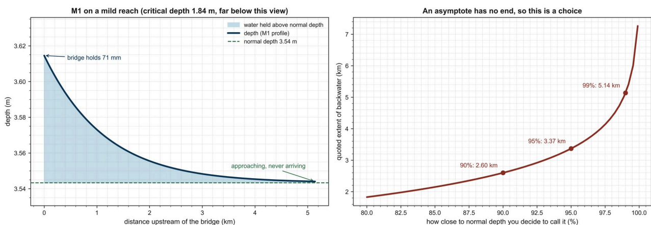
Figure 14.1: The backwater profile and the extent convention. Depth, not level, is plotted, because the bed rises 4 m over the reach while the depth changes by 7 cm.
