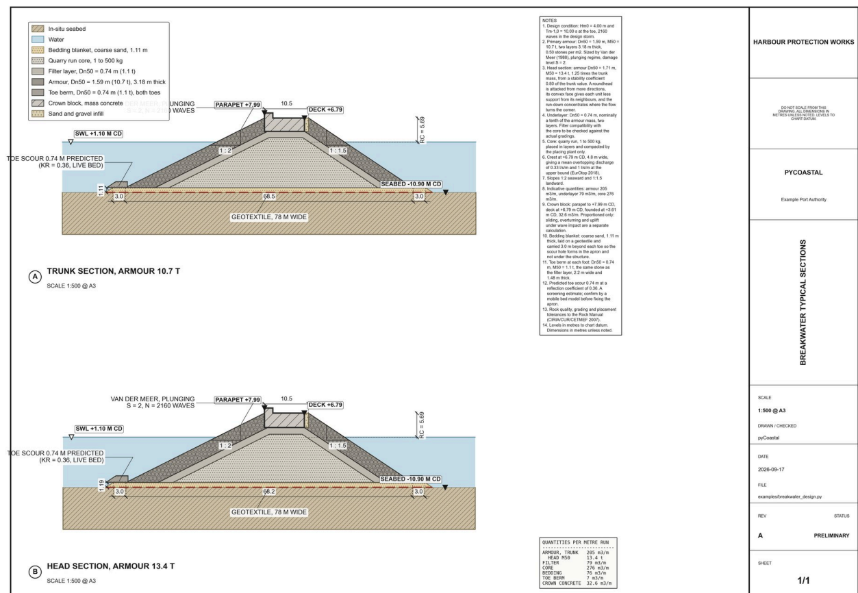
Figure 9.2: The same design issued as a drawing sheet: trunk and head sections with the armor drawn as individual stones at the computed D_{n50} , the bedding blanket, toe berms, crown wall, and generated specification notes.
