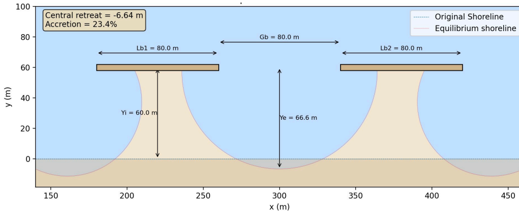
Figure 5.3: Equilibrium shoreline behind two detached breakwaters ( examples/equilibrium_shoreline.py ).
