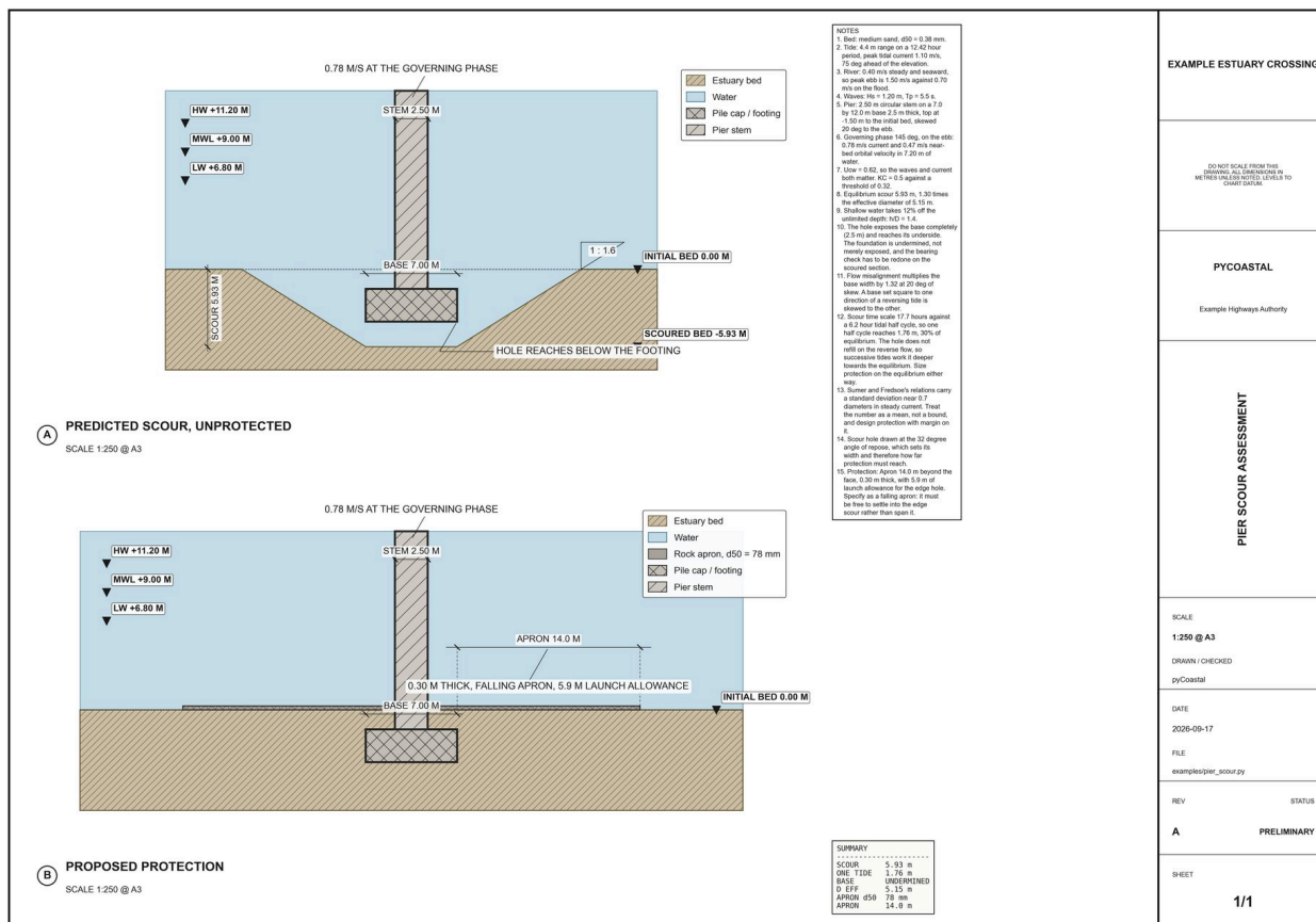
Figure 19.5: Pier scour, unprotected and protected (pier_scour_sheet).
