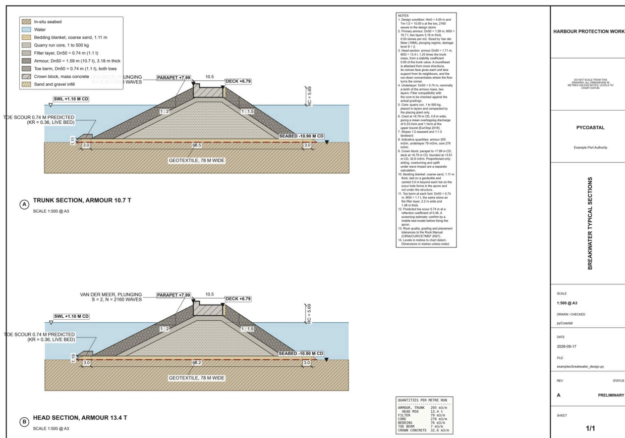
Figure 19.2: Breakwater trunk and head sections (rubb1e_mound_sheet).
