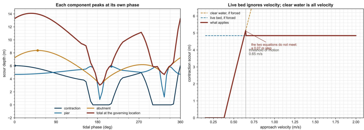
Figure 13.4: Scour components through the tidal cycle. They peak at different phases, so each has its own envelope.
