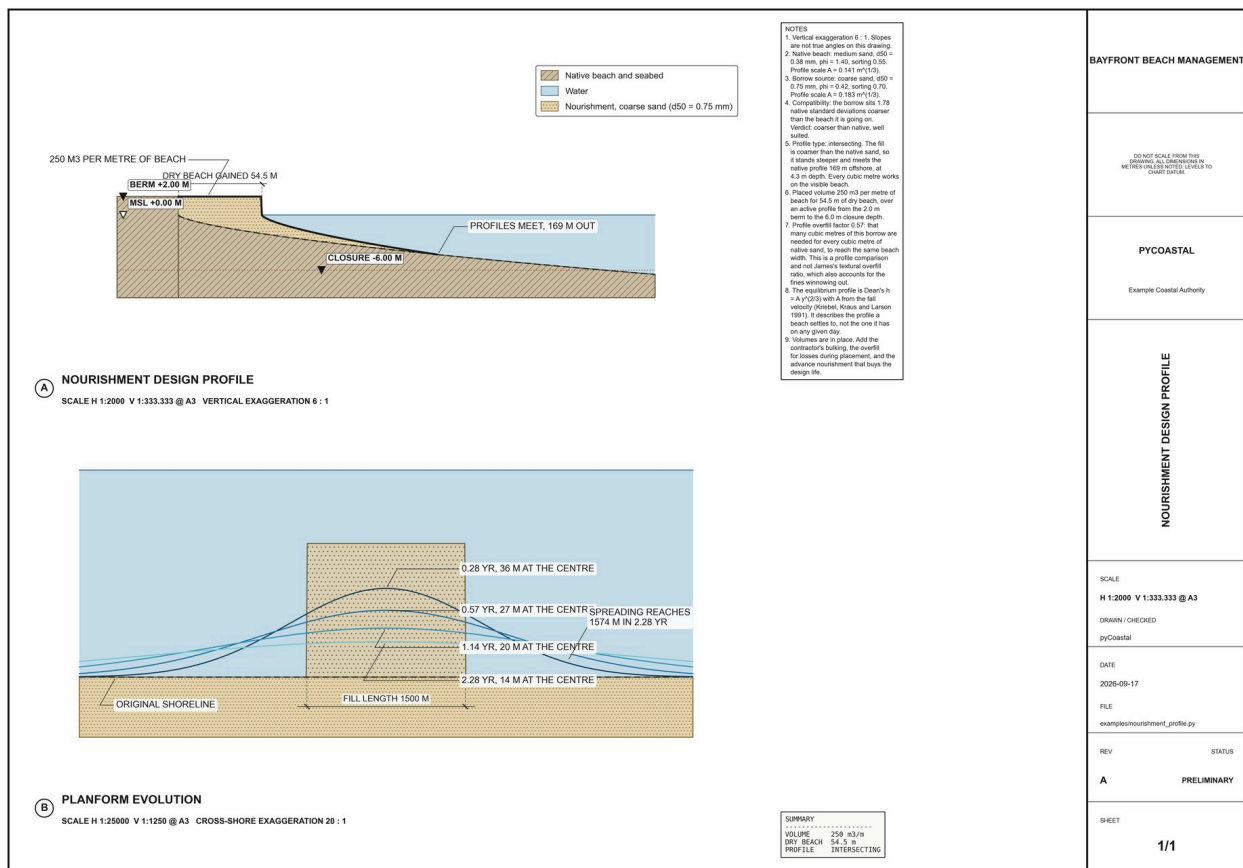
Figure 19.4: Nourishment design profile and planform (nourishment_sheet).
