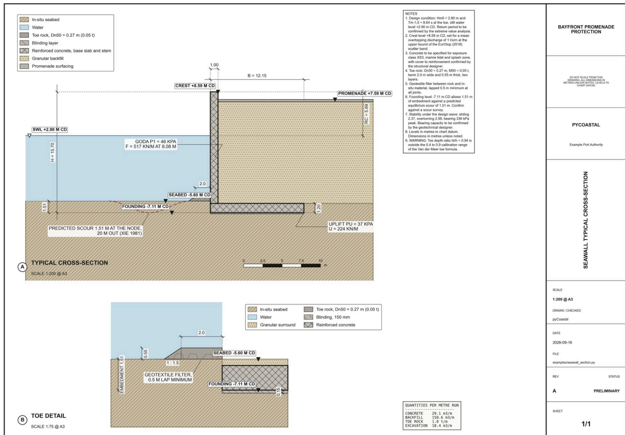
Figure 19.1: Seawall typical cross-section with toe detail (seawa11_sheet).
