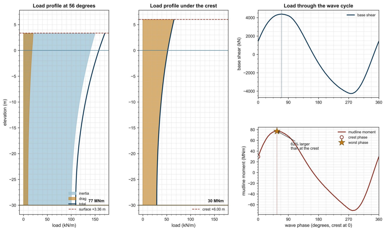
Figure 12.1: Morison loads on an 8 m monopile: load profiles at the crest and worst phases, and force and moment through the wave cycle.
