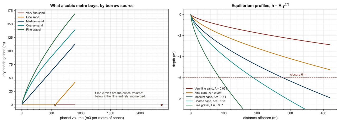
Figure 17.3: The cost of borrow sources: volume per meter of beach for the same dry beach width.
