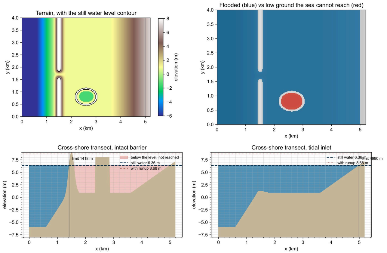
Figure 18.1: Storm surge flood mapping on a barrier-island terrain: threshold-only against connected flooding, with the inlet open and sealed.
