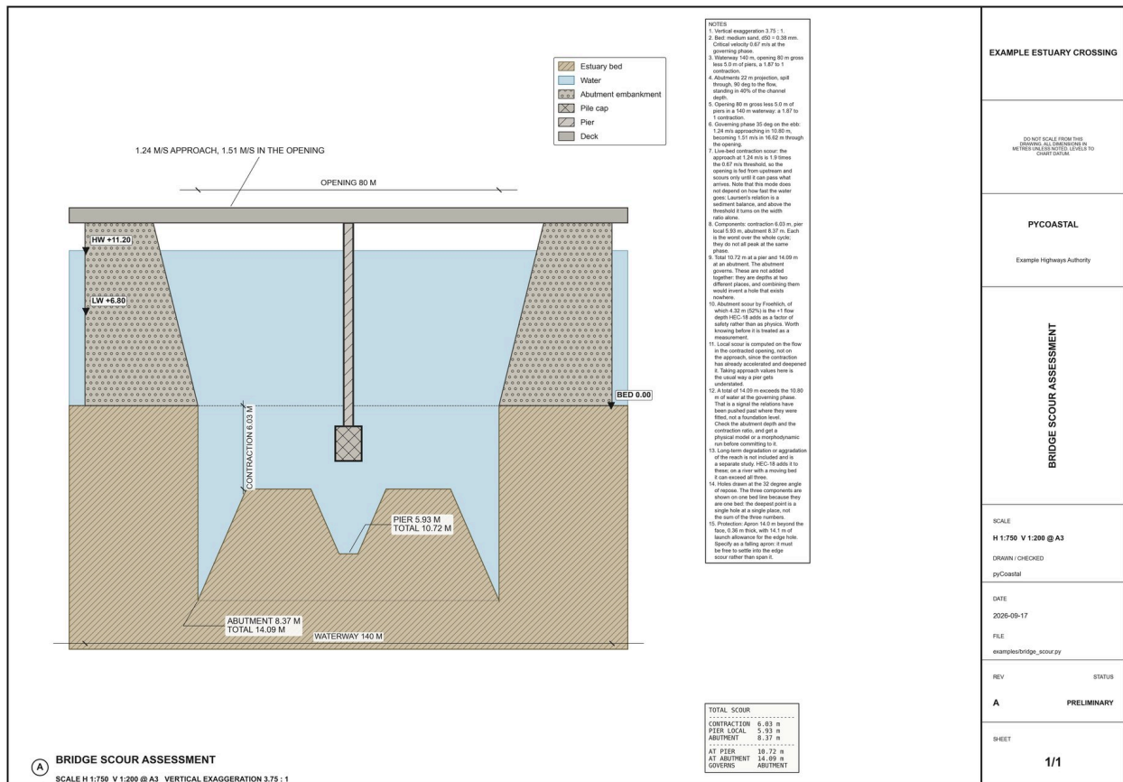
Figure 19.6: Bridge scour, all three components on one bed line (bridge_scor_sheet).
